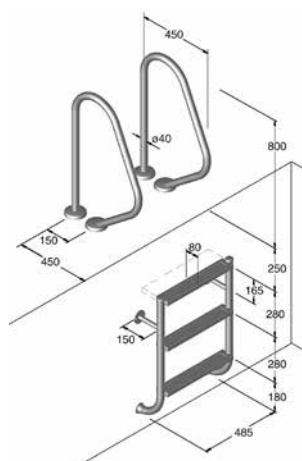
Echelle TINA 2 parties
