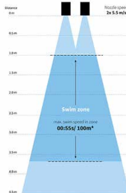
EVASStream MAX double-engine machine
